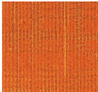
Binary 400006
