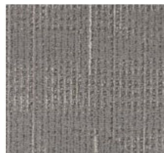
Theorem 400012
