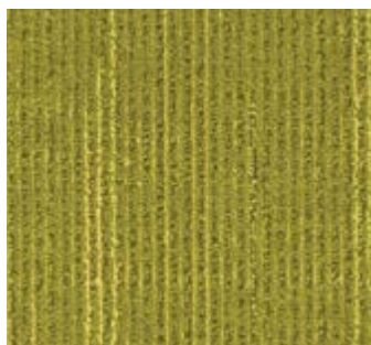
Golden Rectangle 400013
